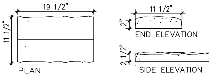
WALL CAP PROFILE
